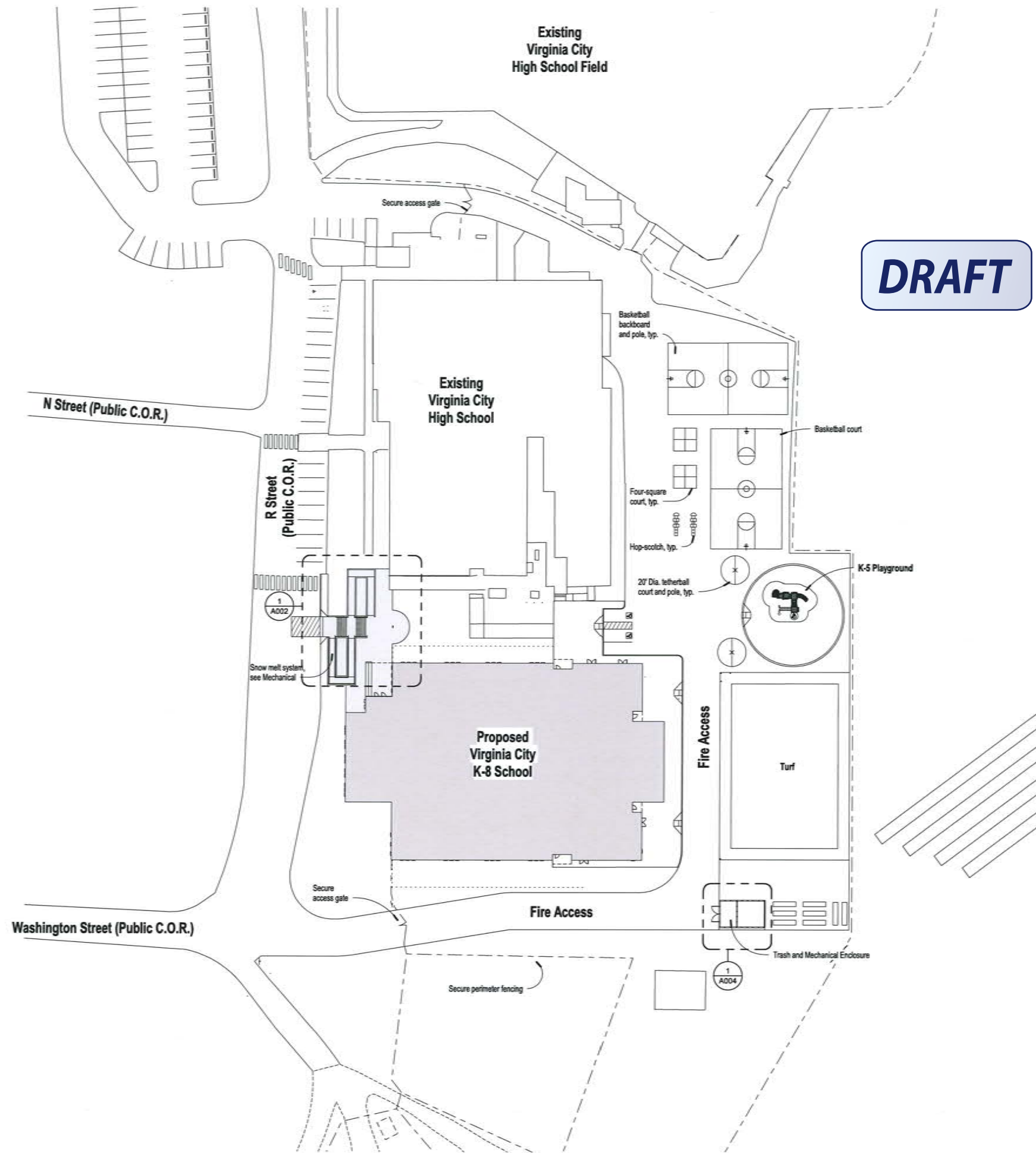
OVERALL SITE PLAN 1" = 80' - 0"
