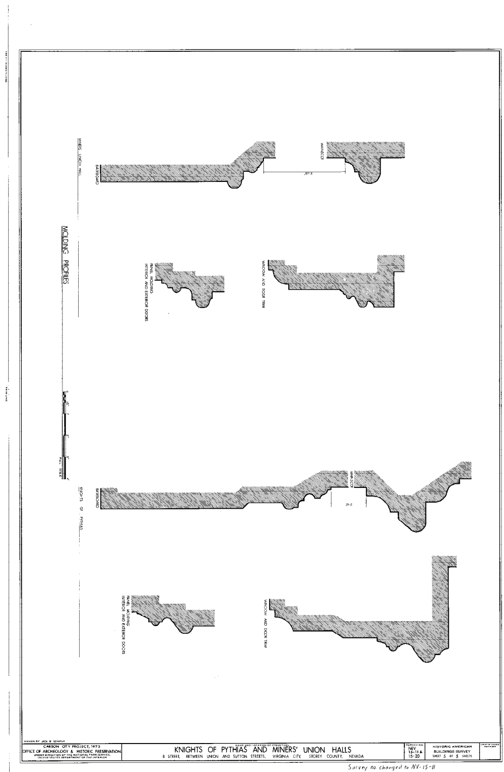
Figure 18. Historic American Buildings Survey drawings illustrating representative molding profiles from the Miners' Union Hall and adjacent Knights of Pythias Hall, including baseboards, wainscoting, window and door trim, and interior and exterior door panel moldings. Courtesy of the Library of Congress (HABS No. NV-15-11, Sheet 5 of 5).
