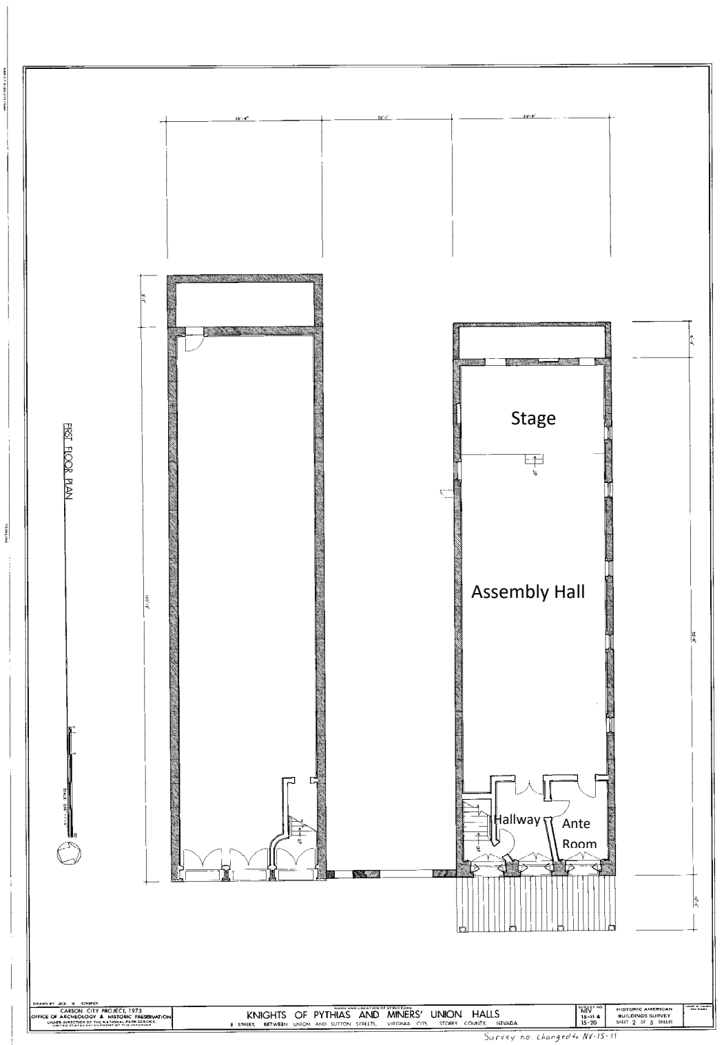
Figure 15. First-floor plan of the Miners' Union Hall and adjacent Knights of Pythias Hall prepared for the Historic American Buildings Survey, illustrating the arrangement of the principal assembly spaces, stage area, entrance vestibules, and circulation patterns. Courtesy of the Library of Congress (HABS No. NV-15-11, Sheet 2 of 5).
