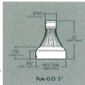
POLE BASE CAP HBC2
