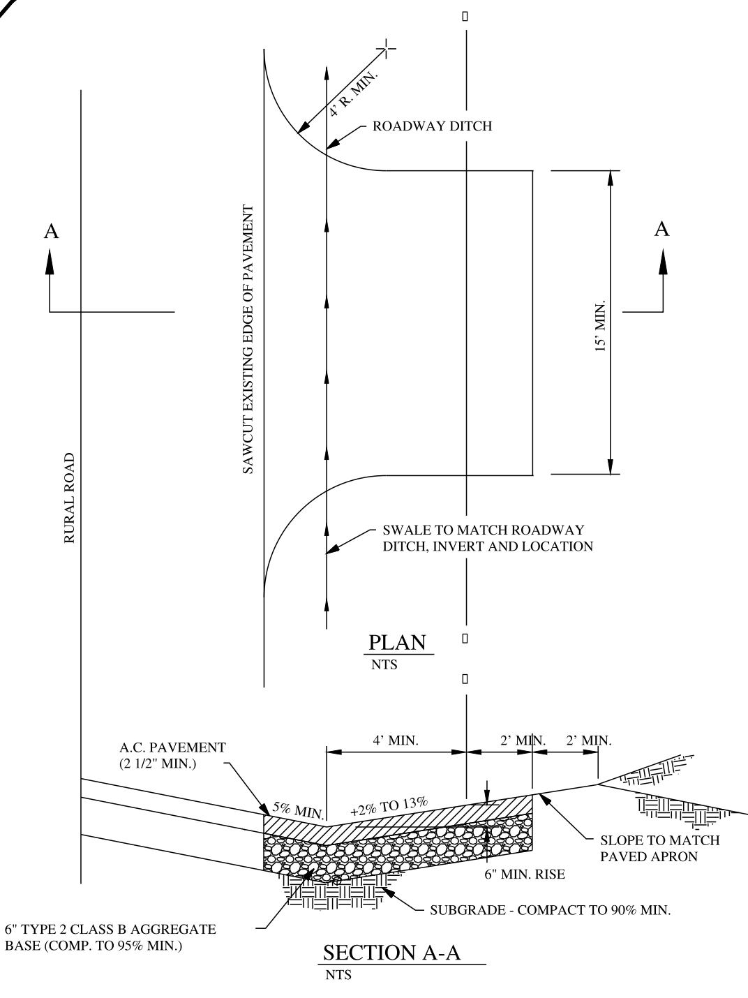
A.C. DRIVEWAY APRON RURAL ROADS
